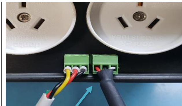
From right-hand port of Exp Unit 1..
